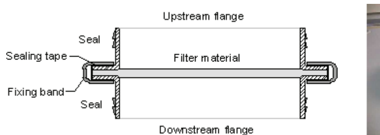
Figure 1. Principle of the sample adapter.
