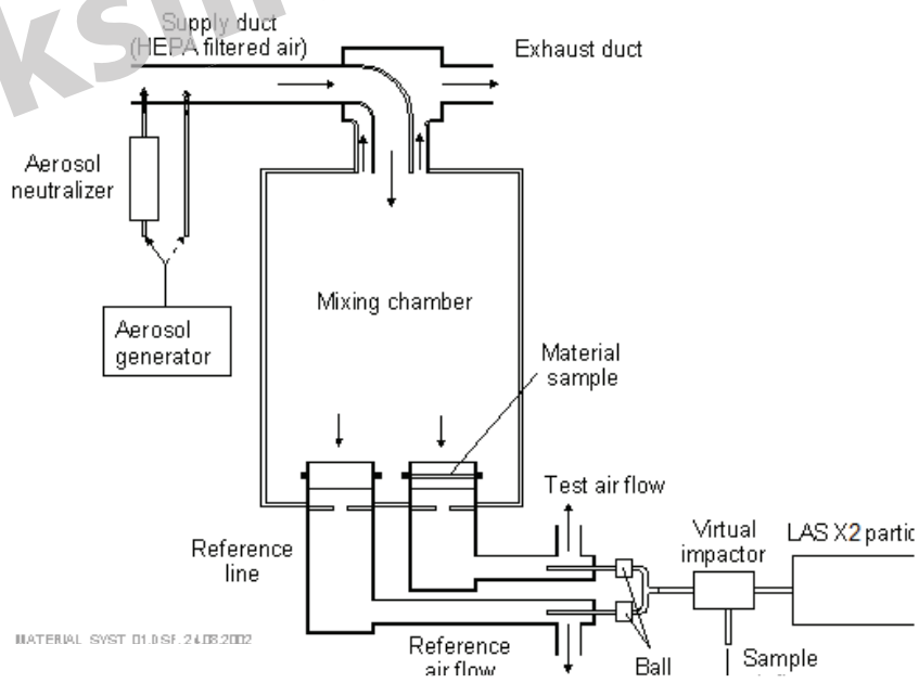
Figure 2. Principle of the test system.
